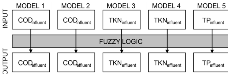
Fig. 2. Inputs and outputs of the fuzzy models
