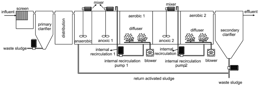
Fig. 1. Schematic diagram of the developed pilot-scale treatment plant [7]
