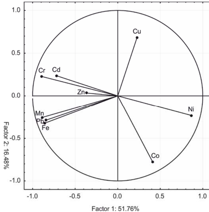
Fig. 1. Content of trace elements in the soils illustrated by the PCA method: vectors represent the analyzed variables (content of Cu, Cd, Pb, Cr, Zn, Ni, Mn, Fe and Co)
