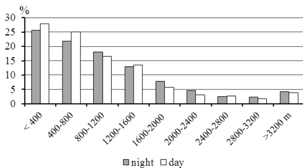
Fig. 4. The base of the elevated inversion layers – frequency of the adopted ranges during the period of calendar winter (December–February). Period: (2004/2005)–(2012/2013)
