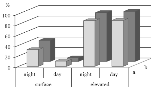
Fig. 2. Frequency of surface and elevated inversion in winter seasons (2004/2005)–(2012/2013) (a), including the days with excessive PM 10 concentration in Gdynia Śródmieście (b)
