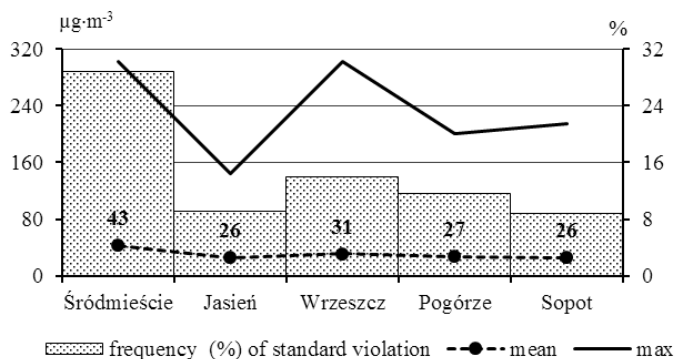
Fig. 1. Characteristics of daily PM 10 concentration in calendar winter (December–February): – mean, maximum and frequency of standard violation. Period: (2004/2005)–(2012/2013)
