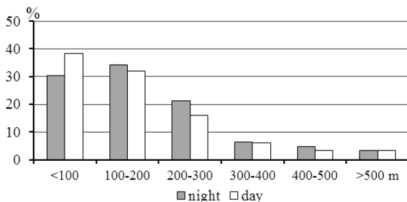
Fig. 5. Thickness of the first (located at the lowest level) elevated inversion layer – frequency of the adopted ranges during the period of calendar winter (December–February). Period: (2004/2005)–(2012/2013)
