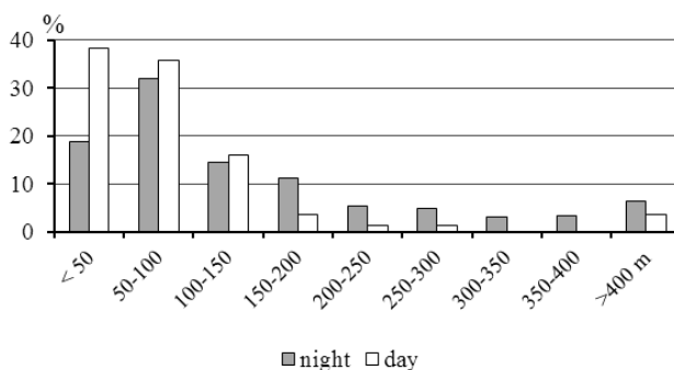
Fig. 3. Thickness of lower layers of inversion – frequency of the adopted ranges during the period of calendar winter (December–February). Period: (2004/2005)–(2012/2013).
